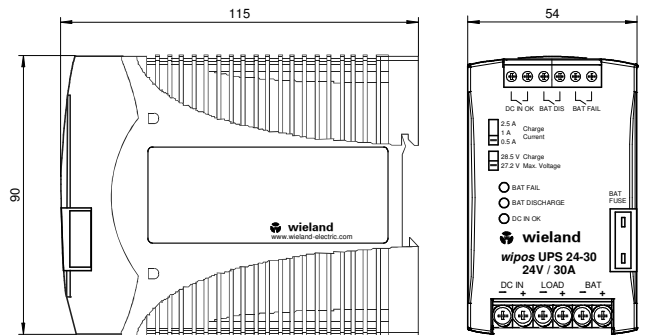
Dimensional diagram
